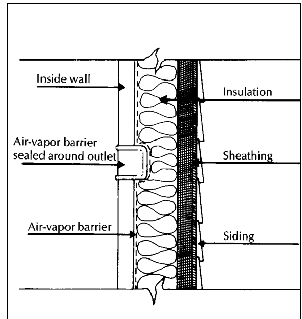
Air-vapor barrier placement
