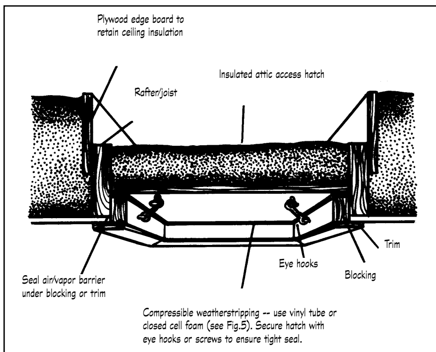
Figure 7: Attic hatches should be sealed to prevent air leakage.
