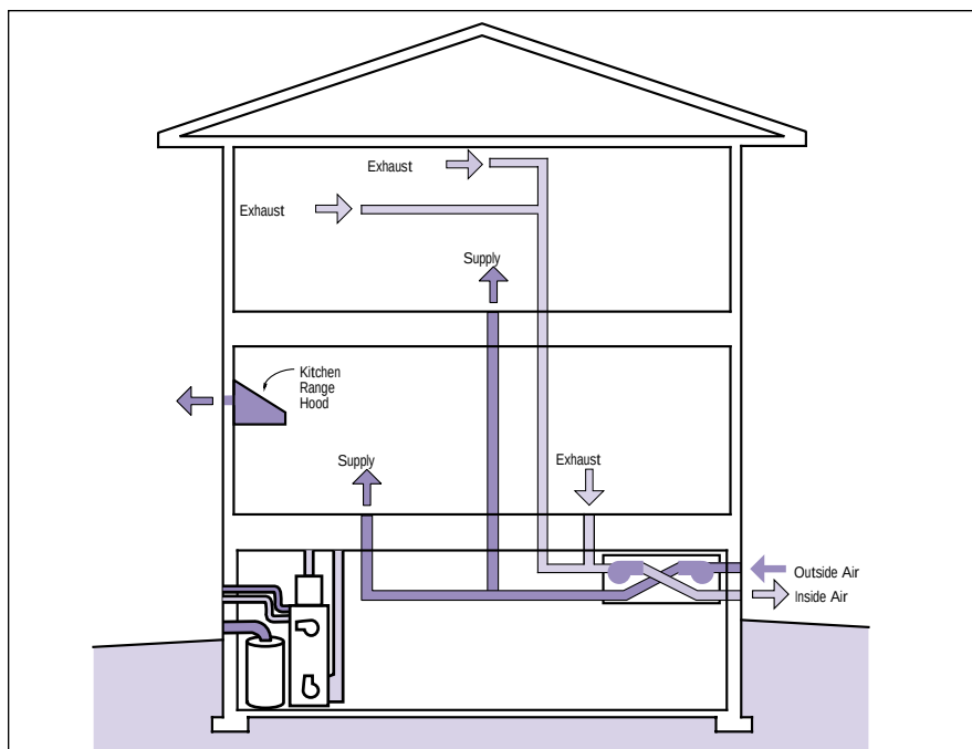
A balanced ventilation system uses power both to exhaust moisture and pollutants to the outside and to bring in fresh air from the outdoors. The furnace and water heater shown in the diagram exhaust their combustion gases outside and bring in combustion air without mixing them with indoor air.
