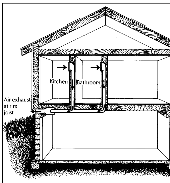
Figure 5 Mechanical ventilation
