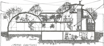
CROSS SECTION
