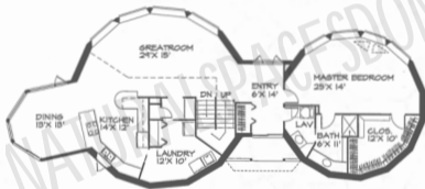
MAIN FLOOR 1420 SQ. FT.
