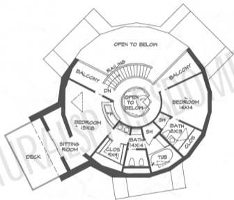
UPPER FLOOR MAIN DOME 1000 SQ. FT.
