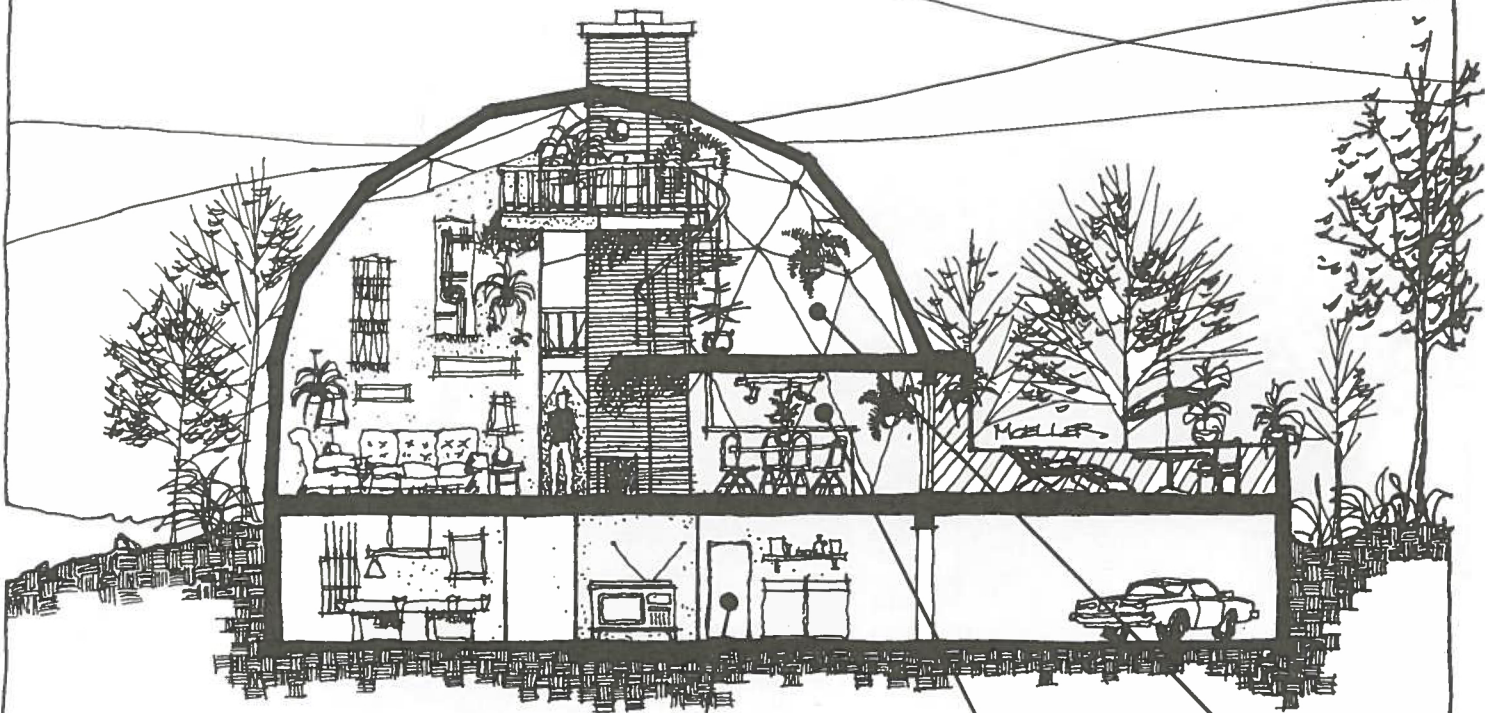
CROSS SECTION
