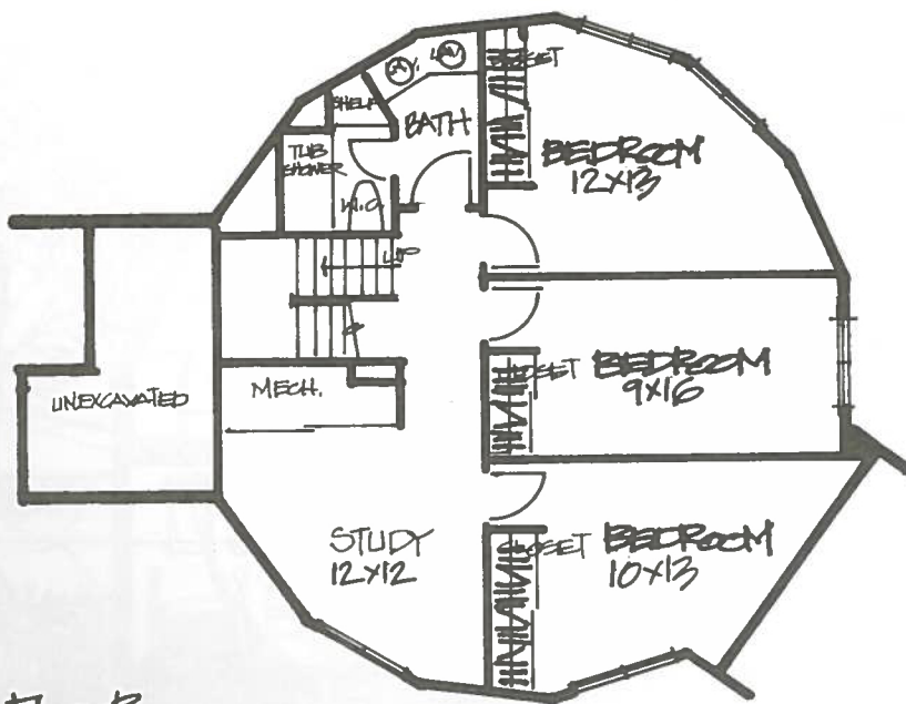
LOWER FLOOR 950 SQ. FT.
